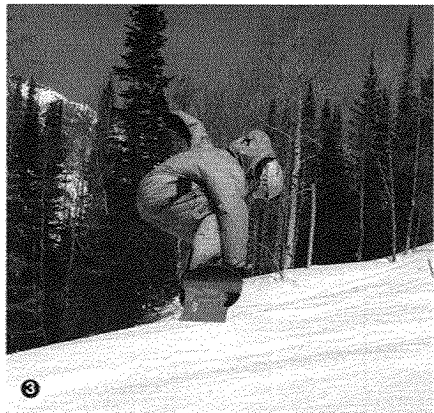
The 180 maneuver
