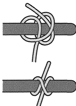
Clove hitch
