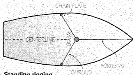
Standing rigging
