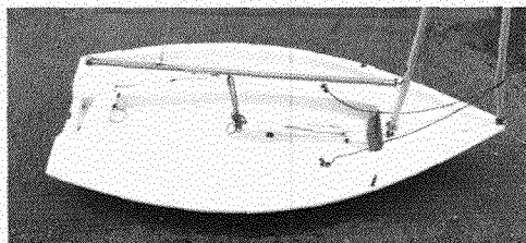
Standing rigging, side view
