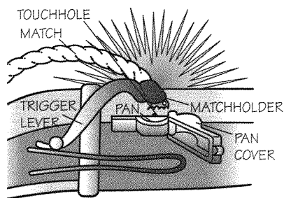
Matchlock action
