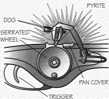
Wheel lock action
