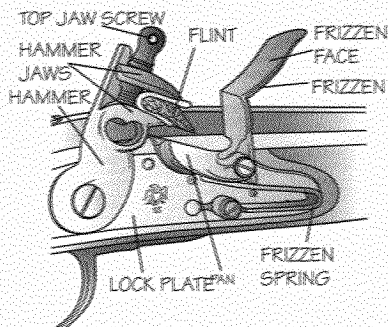
Flintlock action
