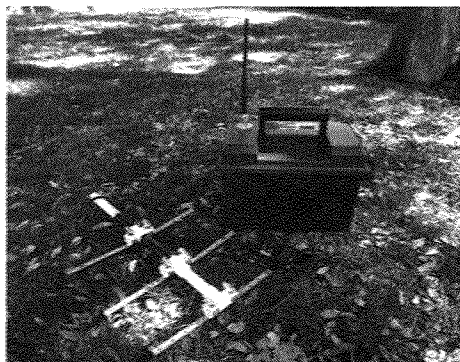
A 2-meter receiver/antenna and transmitter
