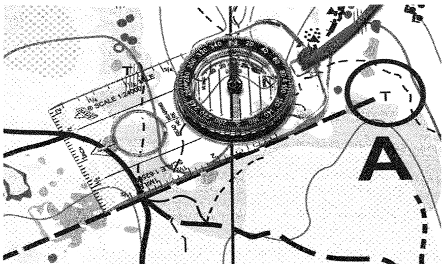
On the Sid Richardson Scout Ranch map, the compass edge is laid alongside the line from the hunter's stand at "A" and the northwest end of the cliff at "B." The bezel is turned until the north-south lines within the ring line up with the north arrow of the compass. Read the bearing from the index. The bearing is 244 degrees from "A" to "B." (Points "A" and "B" can be seen in the top photo on page 21.)
