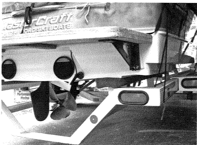
Inboard motor
