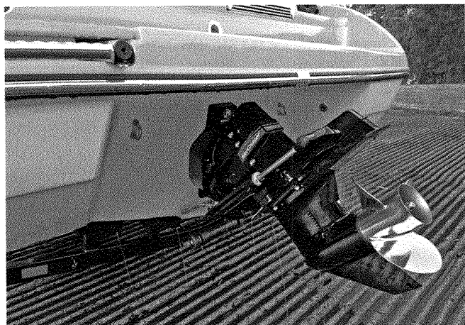
Inboard/outboard motor
