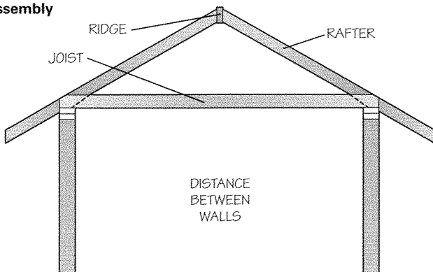
Ceiling joist
