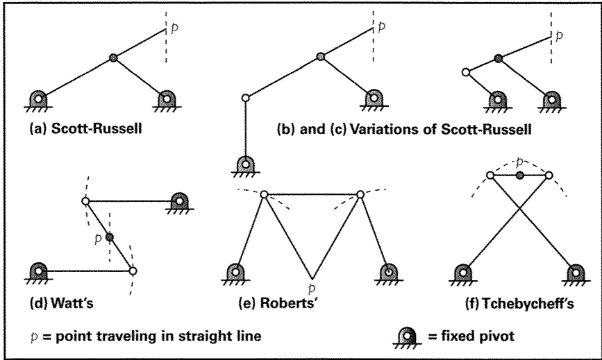
Straight-line mechanisms
