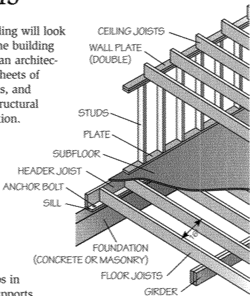
Framing
