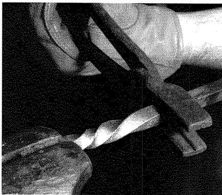
Bending steel over the edge of the anvil creates L-shaped bends.
