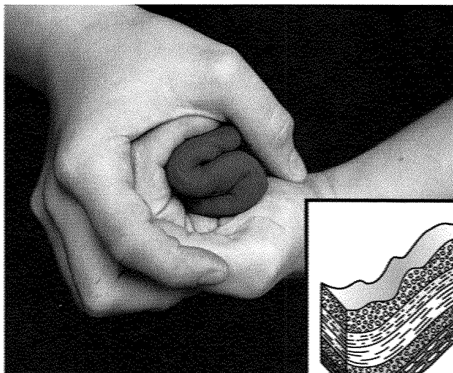
Folds
