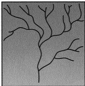
Dendritic stream map view
