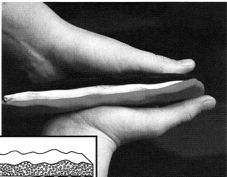
Horizontal layers
