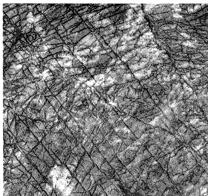
Slate (metamorphic)
