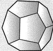
Pyrite
