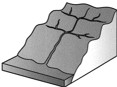
Trellis stream perspective view
