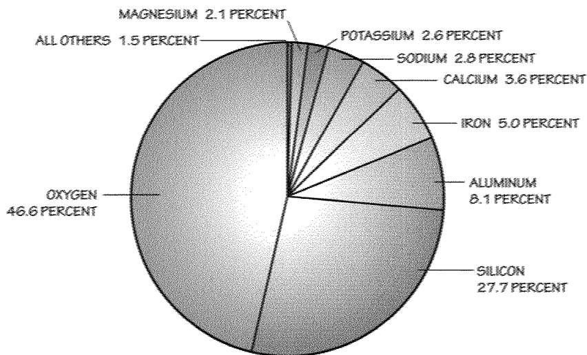
Relative abundance of elements in Earth's crust
