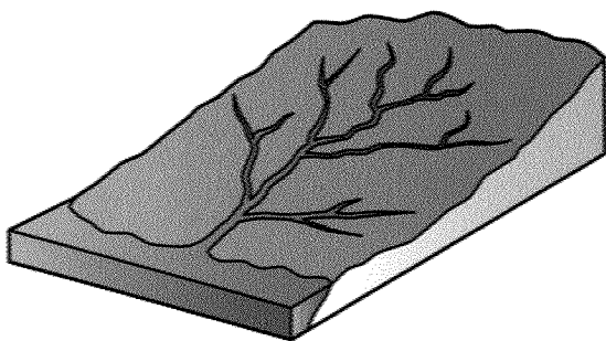
Dendritic stream perspective view
