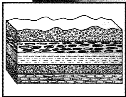
Horizontal layers
