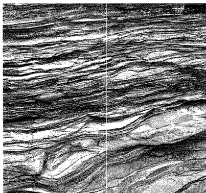
Shale (sedimentary)
