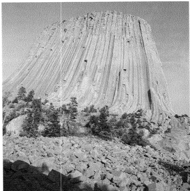
Devils Tower in Wyoming shoots upward in basalt pillars, an igneous rock.
