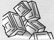
Halite
