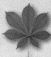
Compound
