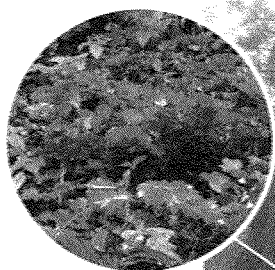
SHRUB LAYER
