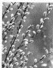
Pussy willows
