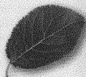
Toothed edge
