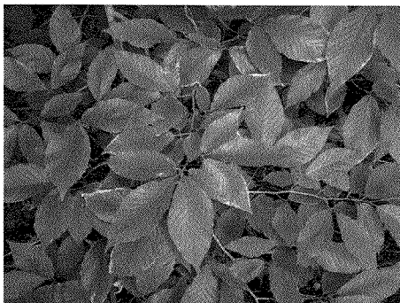
American beech
