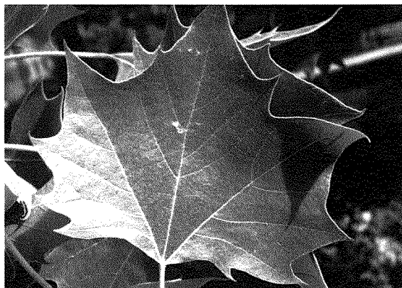
American sycamore
