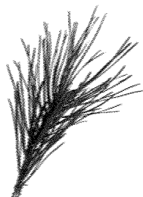
White pine
