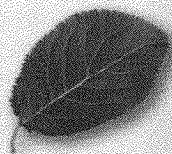
Unlobed
