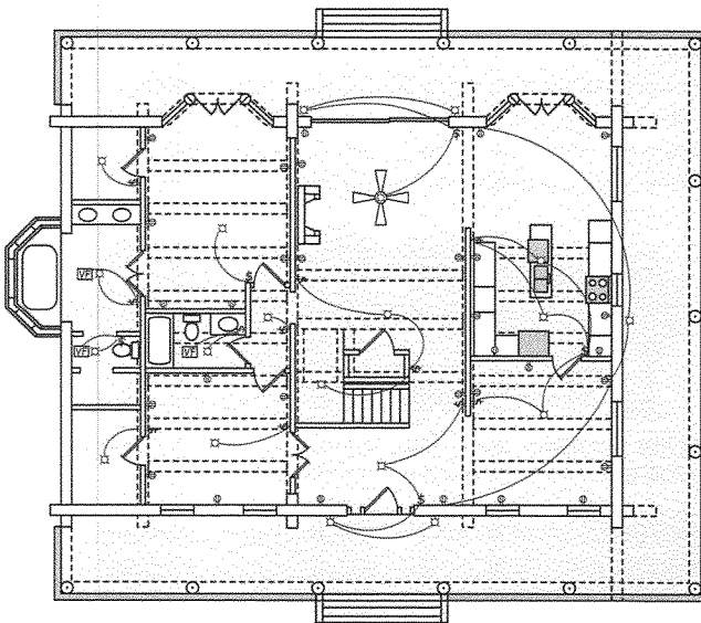
Electrical plan
