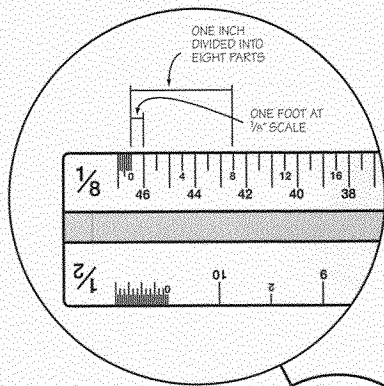
ENLARGEMENT OF \frac{1}{8} " SCALE
