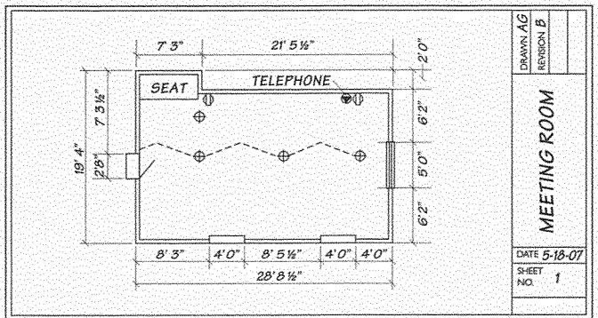
The sketch redrawn to scale using drafting instruments, and neatly lettered
