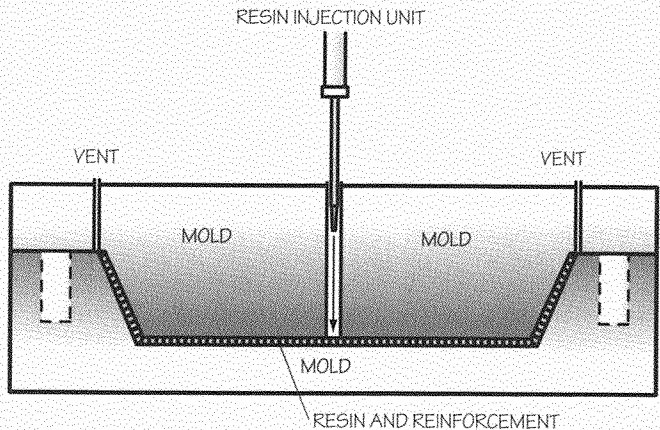
Resin transfer molding processes
