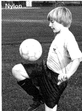
Nylon
