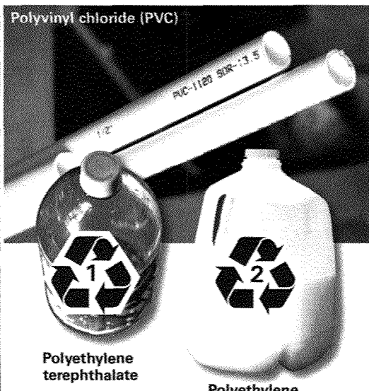
Polyethylene
