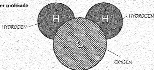
Water molecule
