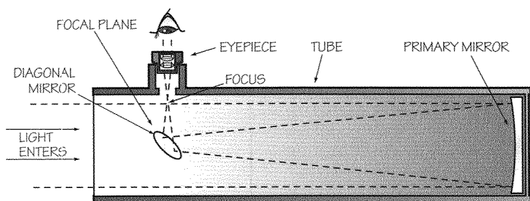
Principle of a reflecting telescope
