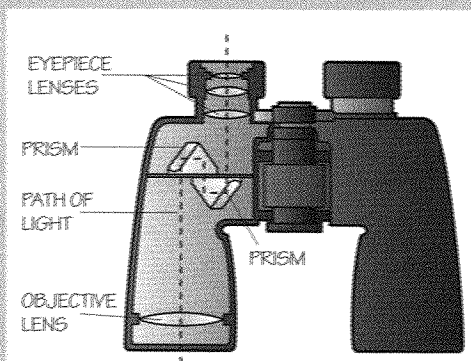
Standard binoculars
