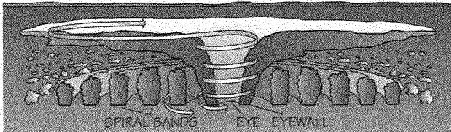
Cross section showing the structure of a typical mature tropical cyclone
