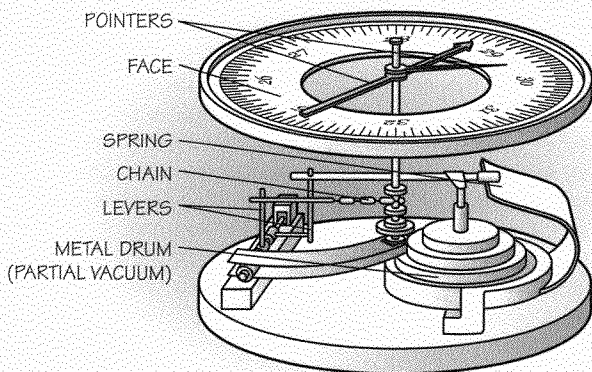
Changes in pressure result in changes in width of an aneroid barometer's sealed box. Levers and springs convert these changes into pressure readings.
