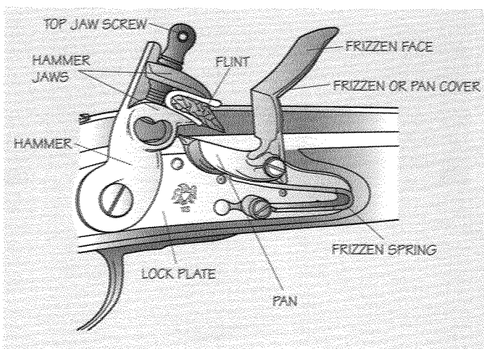
Flintlock action
